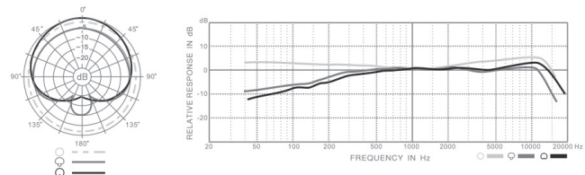
E309D PRO Frequency Response
